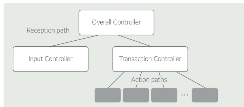
[Figure 16] Structure of the program based on transactions
