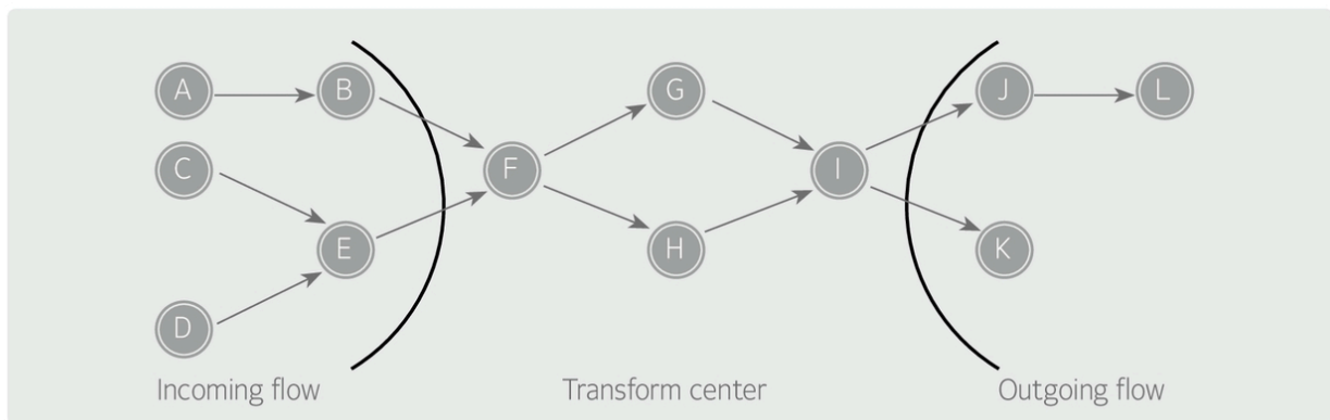
[Figure 13] Input and output boundary of the data flow diagram
