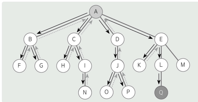
[Figure 9] Example of depth first search
