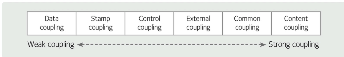
[Figure 12] Type and degree of coupling
