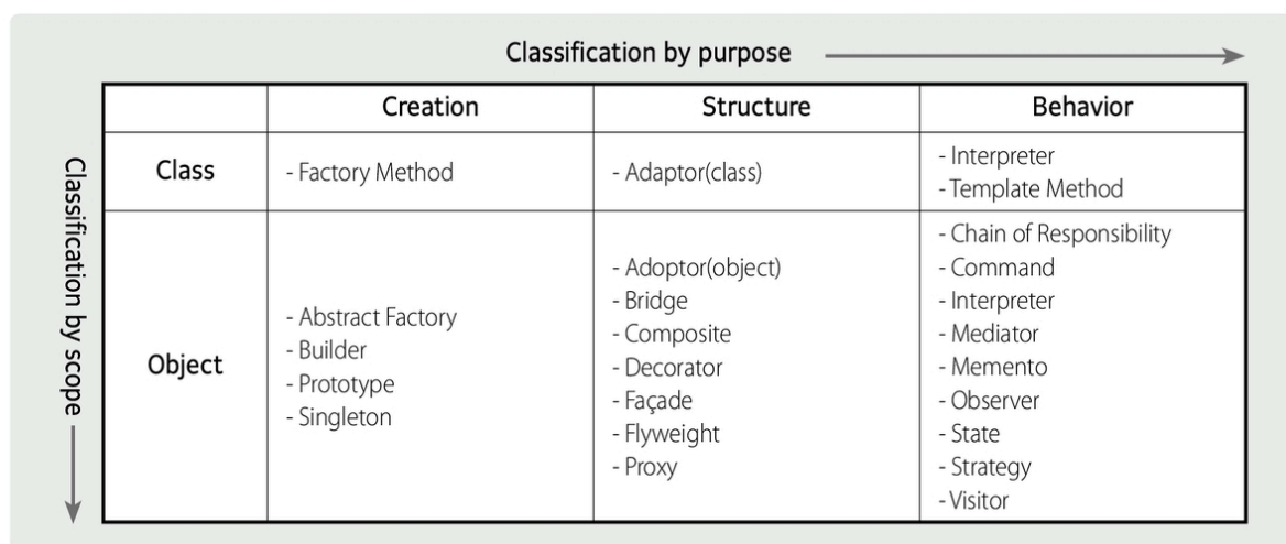
[Figure 18] Classification of design patterns
