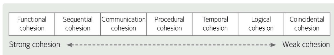
[Figure 11] Type and degree of cohesion
