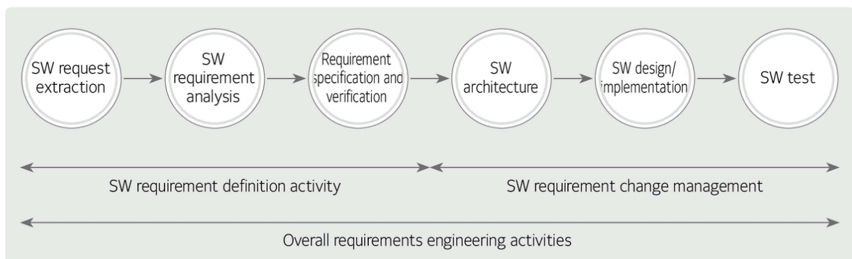
[Figure 24] Requirements management activities
