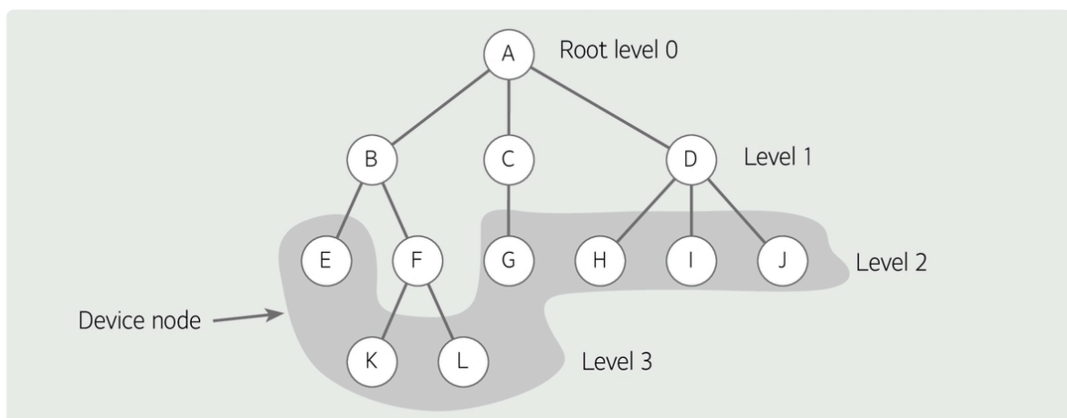
[Figure 4] Conceptual diagram of the tree
