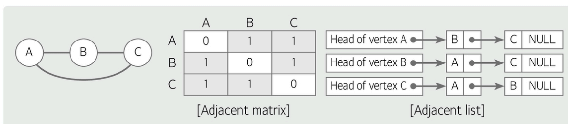
[Figure 5] Graphing method
