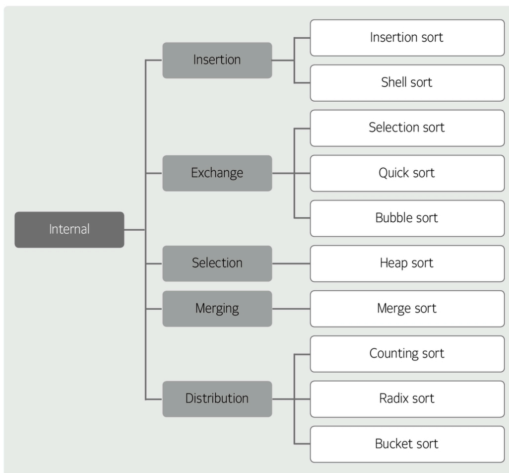
[Figure 6] Classification of internal sorting algorithms
