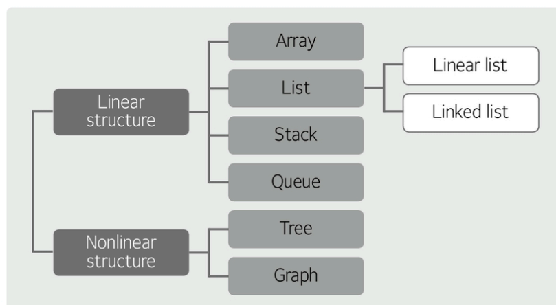
[Figure 1] Classification of the data structure
