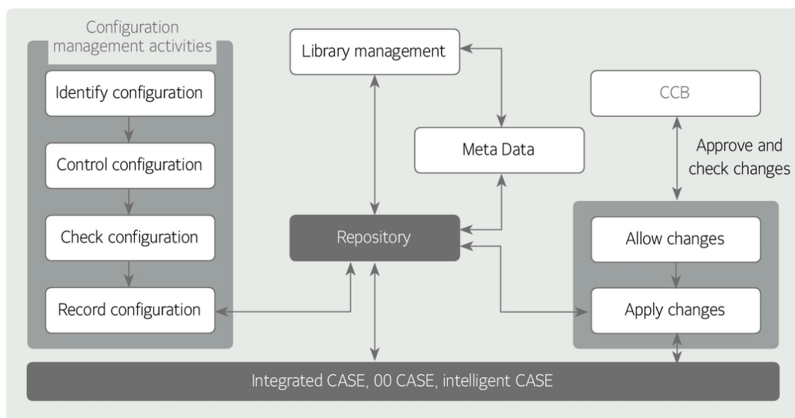
[Figure 26] Conceptual diagram of configuration management
