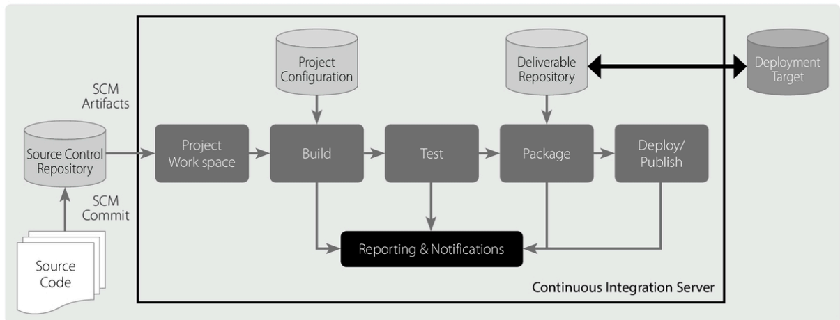
[Figure 22] Composition diagram of CI (Continuous Integration)
