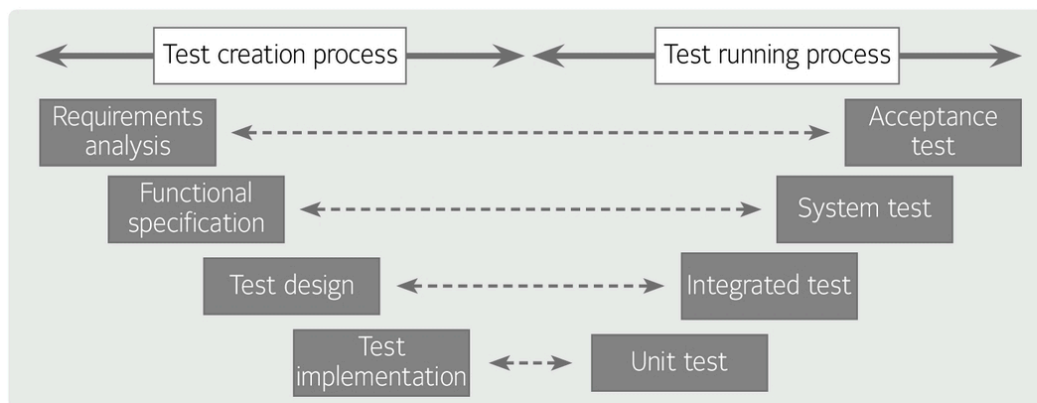
[Figure 23] Test level types
