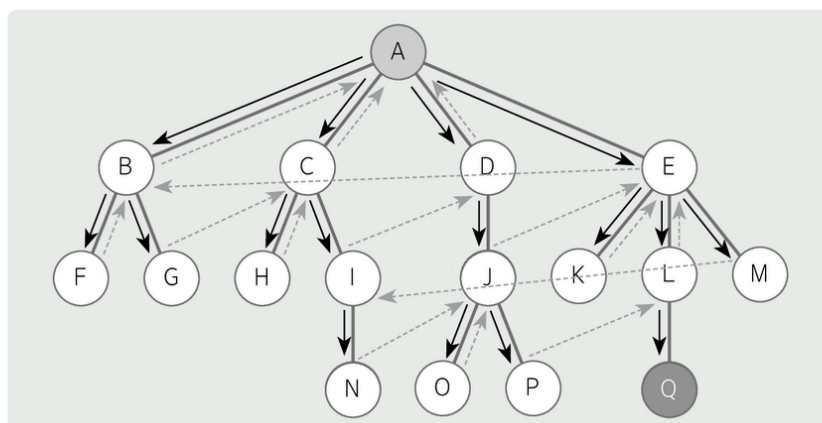
[Figure 10] Example of breadth first search
